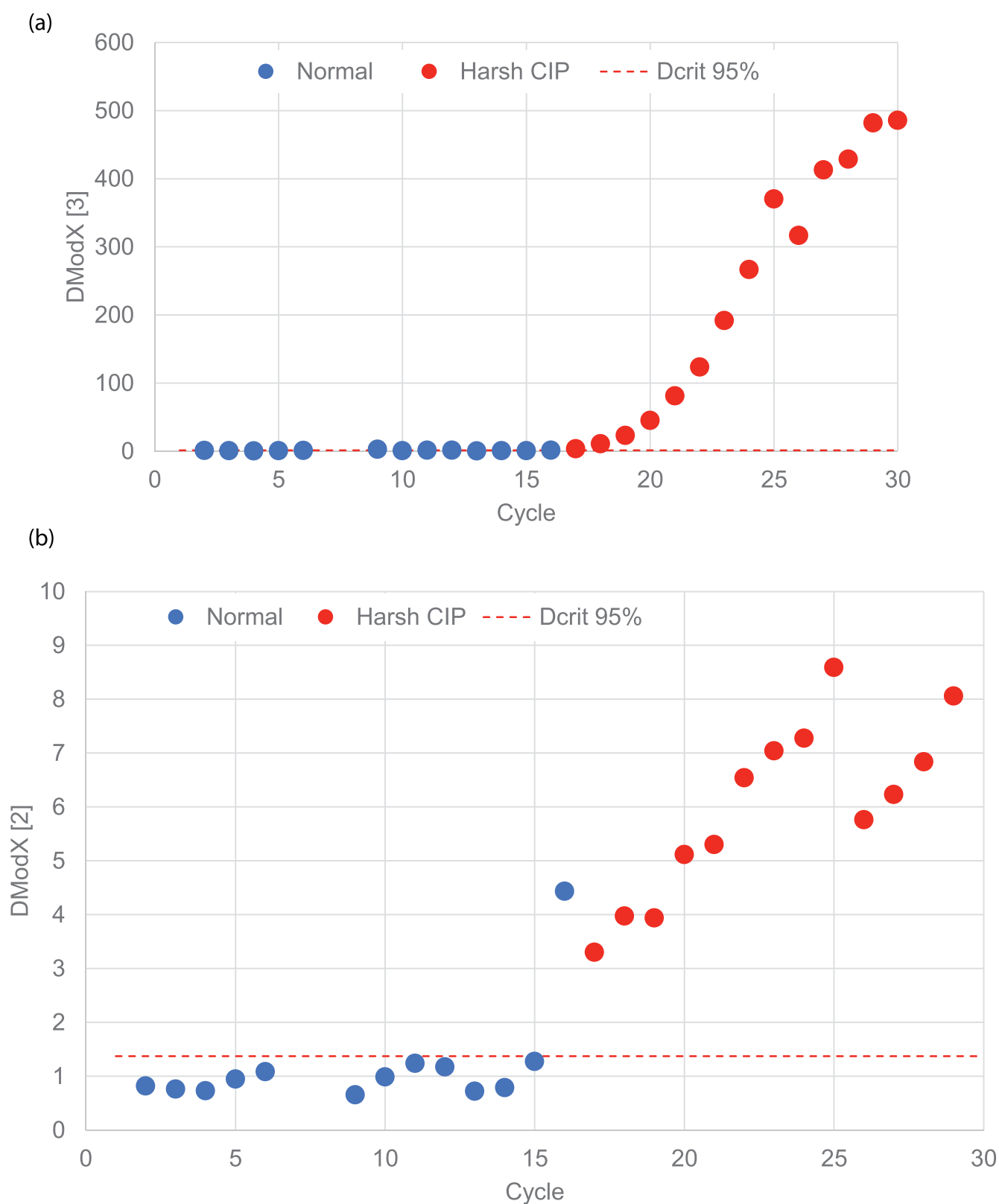
Fig. 9. Distance to model plot for the (a) Wash, (b) Elution at 600 nm and (c) Strip. Cycle 16 is included with the “normal CIP” cycles since the harsh CIP takes place at the end of the chromatography method. Dcrit is 1.371.
