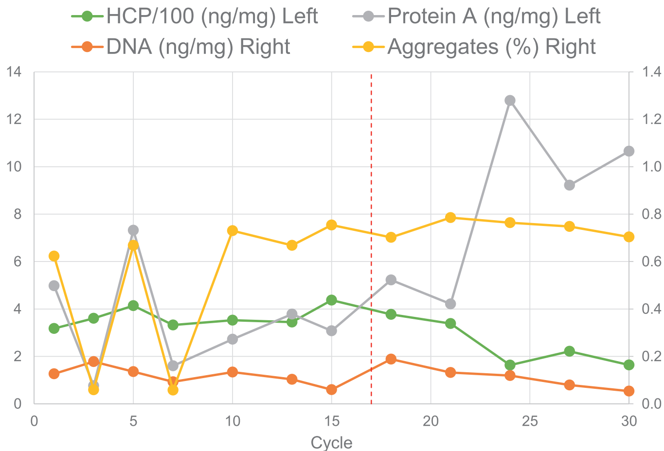
Fig. 4. Product quality for selected chromatography cycles during the normal cycles (1–16) and the harsh CIP cycles (17–30). The red dashed line indicates the change from normal to harsh CIP.
