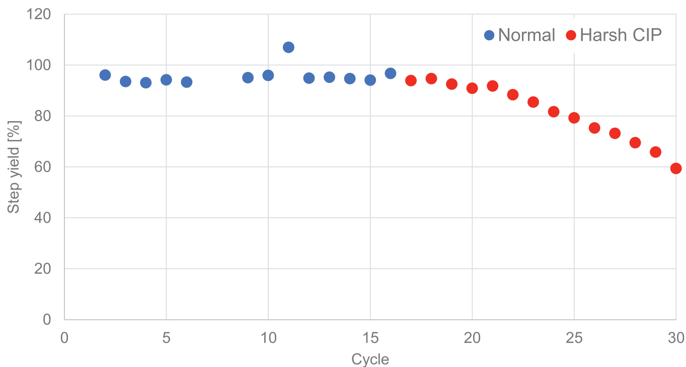
Fig. 2. Step yield measurements over the first 15 chromatography runs using NaOH exposure as recommended by the vendor followed by 15 additional runs which used an harsh CIP.
