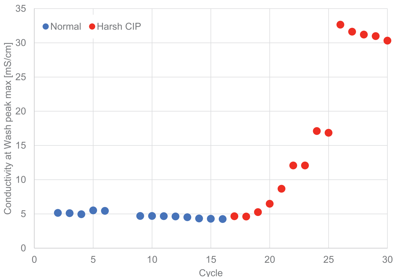
Fig. 12. SOP-MPT analysis of the Wash phase. Outlier cycles 1,7 and 8 excluded.
