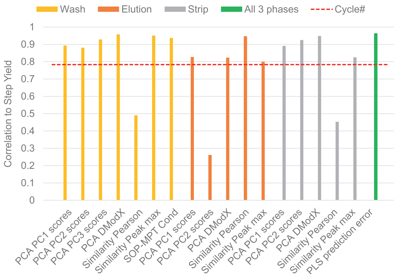
Fig. 13. Comparison of different metrics with respect to the absolute value of the correlation to step yield over the cycles. Only the relevant metrics for each phase are shown. The correlation to Cycle number is used as a cutoff criteria to indicate an improved predictive ability. The metrics are the calculated PCA scores for PC1, PC2 (and PC3 in Wash), PCA distance to model (DModX), similarity score Pearson correlation and peak max, SOP-MPT for conductivity and absolute value of the PLS cycle number prediction error.
