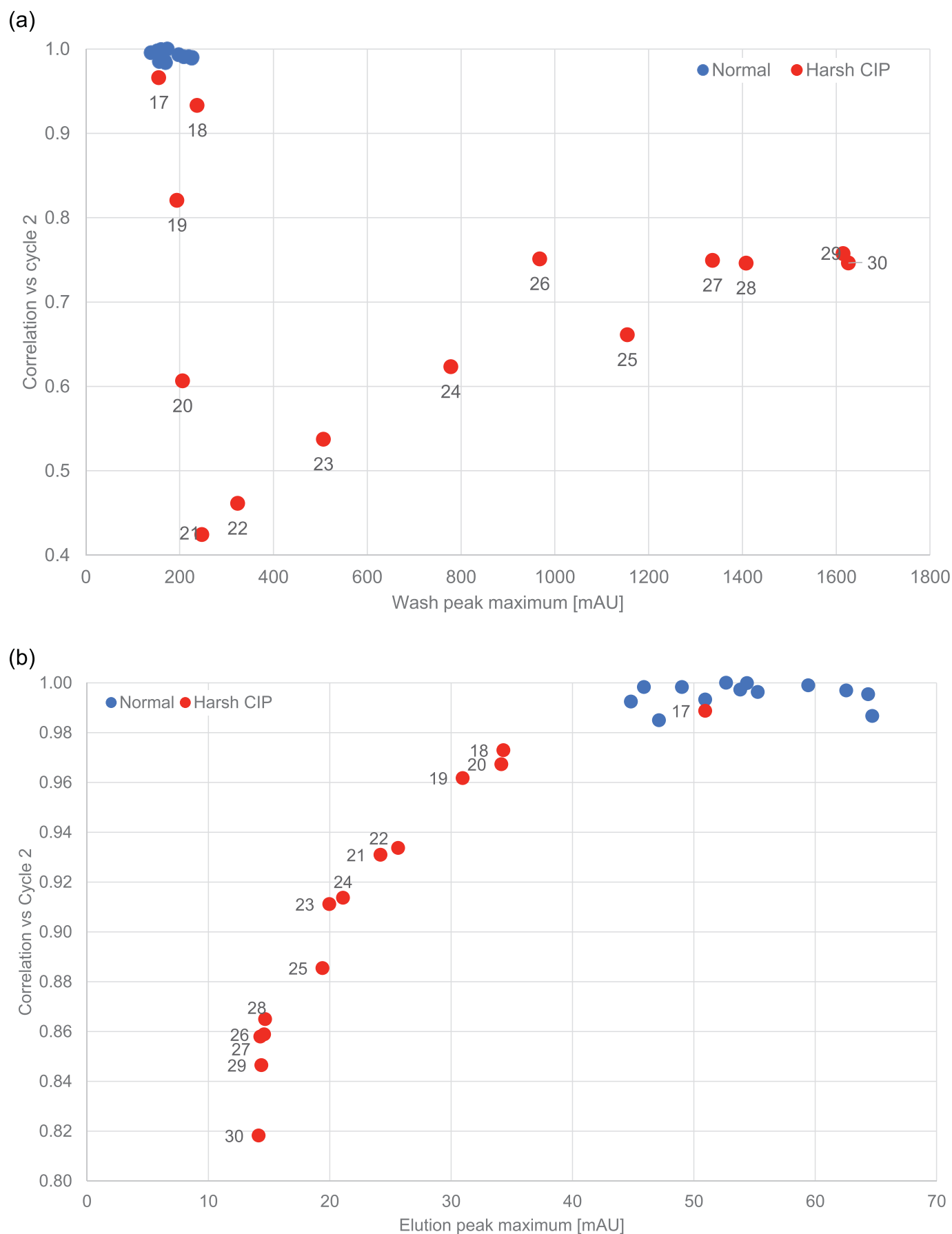
Fig. 11. Similarity Score plot with cycle 2 as reference, for (a) Wash, (b) Elution at 600 nm and (c) Strip. Cycle 16 is included with the “normal CIP” cycles since the harsh CIP takes place at the end of the chromatography method.
