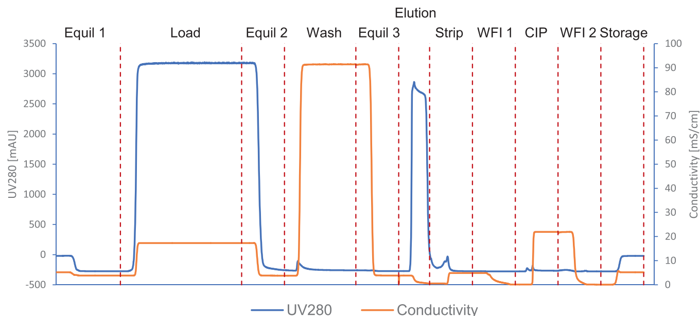
Fig. 1. Typical protein A capture chromatogram with the phase changes indicated by red dashed lines. The traceline for absorbance at 280 nm reaches saturation level in the Load phase and in the Elution. The buffer used in Equil 1, Equil 2 and Equil 3 was Tris-based and had neutral pH. The Wash used a high NaCl content buffer also at neutral conditions. Elution used an acetate-based buffer at low pH. The resin was regenerated with a combination of acidic buffer (Strip) and NaOH solution (CIP).
