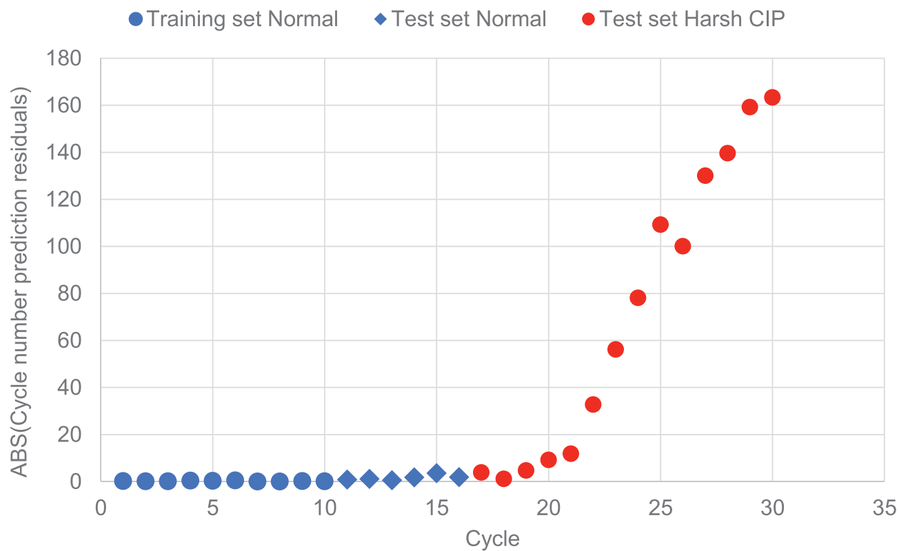
Fig. 10. The results of supervised modeling: a PLS model was trained to predict the cycle number, with the initial 10 cycles used as a training set, and the remaining 20 cycles as a test set. The predictions are consistent with the actual cycle number until cycle 18, after which they become progressively worse as shown by the absolute values of the prediction error.
