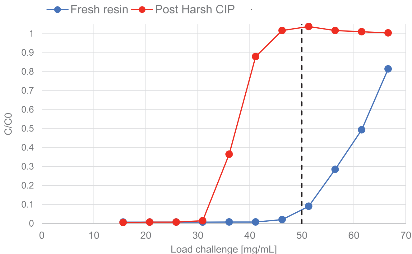
Fig. 3. Dynamic binding capacity for fresh resin (pre-run) and after the harsh CIP (post-run). The black dashed line indicates the load challenge during the study (50 mg/mL).
