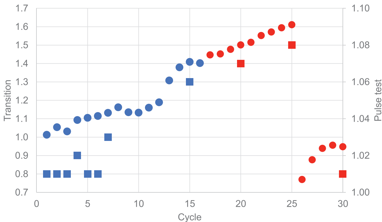
Fig. 6. Comparison of asymmetry data from pulse test (squares) and transition analysis (circles). The normal CIP cycles are indicated by blue symbols and the harsh CIP by red symbols.
