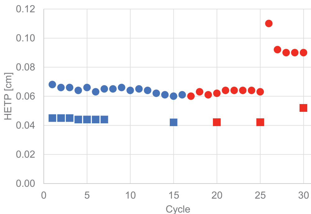
Fig. 5. Comparison of HETP from pulse test (squares) and transition analysis (circles). The normal CIP cycles are indicated by blue symbols and the harsh CIP by red symbols.
